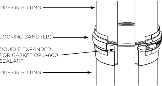
Model SWCK Joint Assembly Detail
