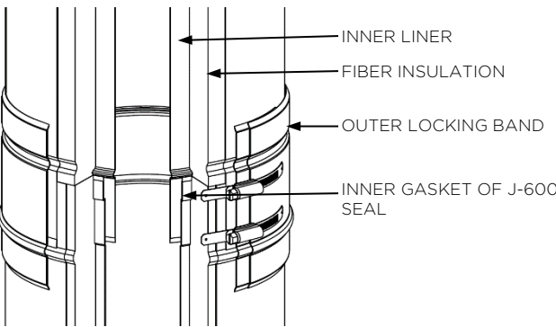
Model DWCK+1 & DWCK-ZC Joint Assembly Detail
